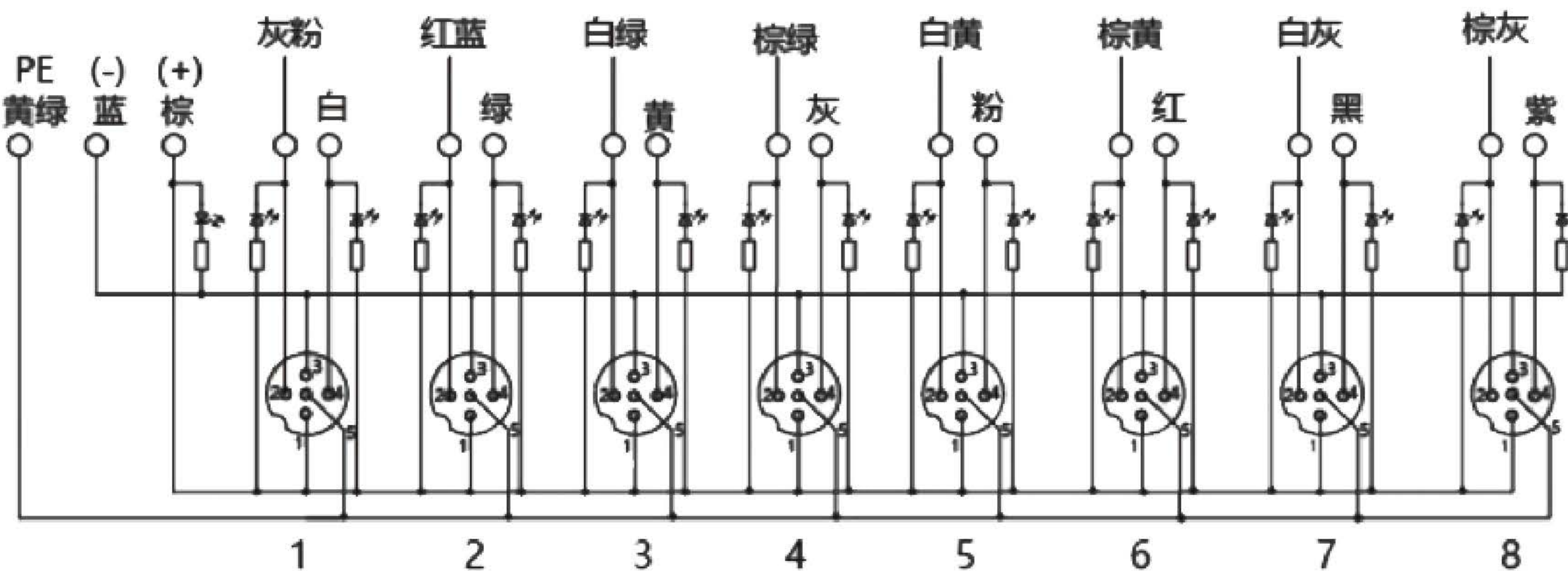
M8/ M12 Distribution Systems
