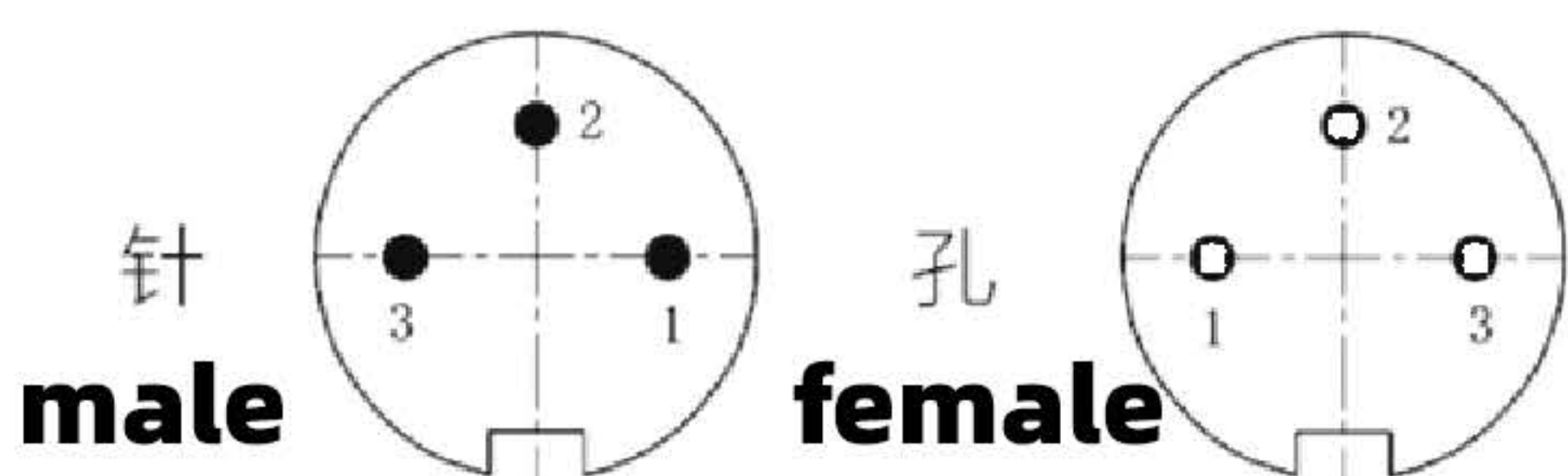
rear male
